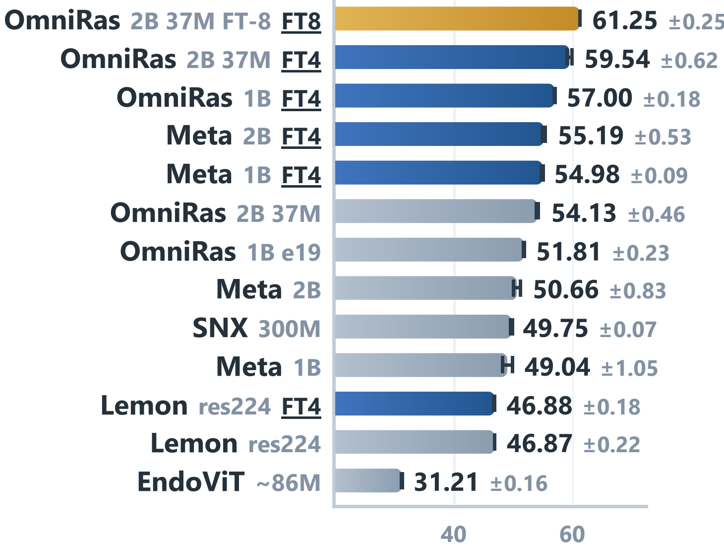
Target mAP
