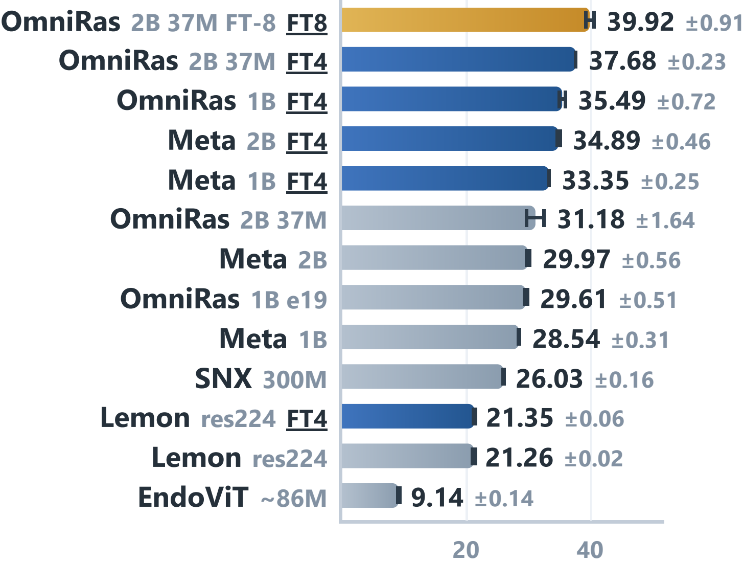
Joint IVT mAP
