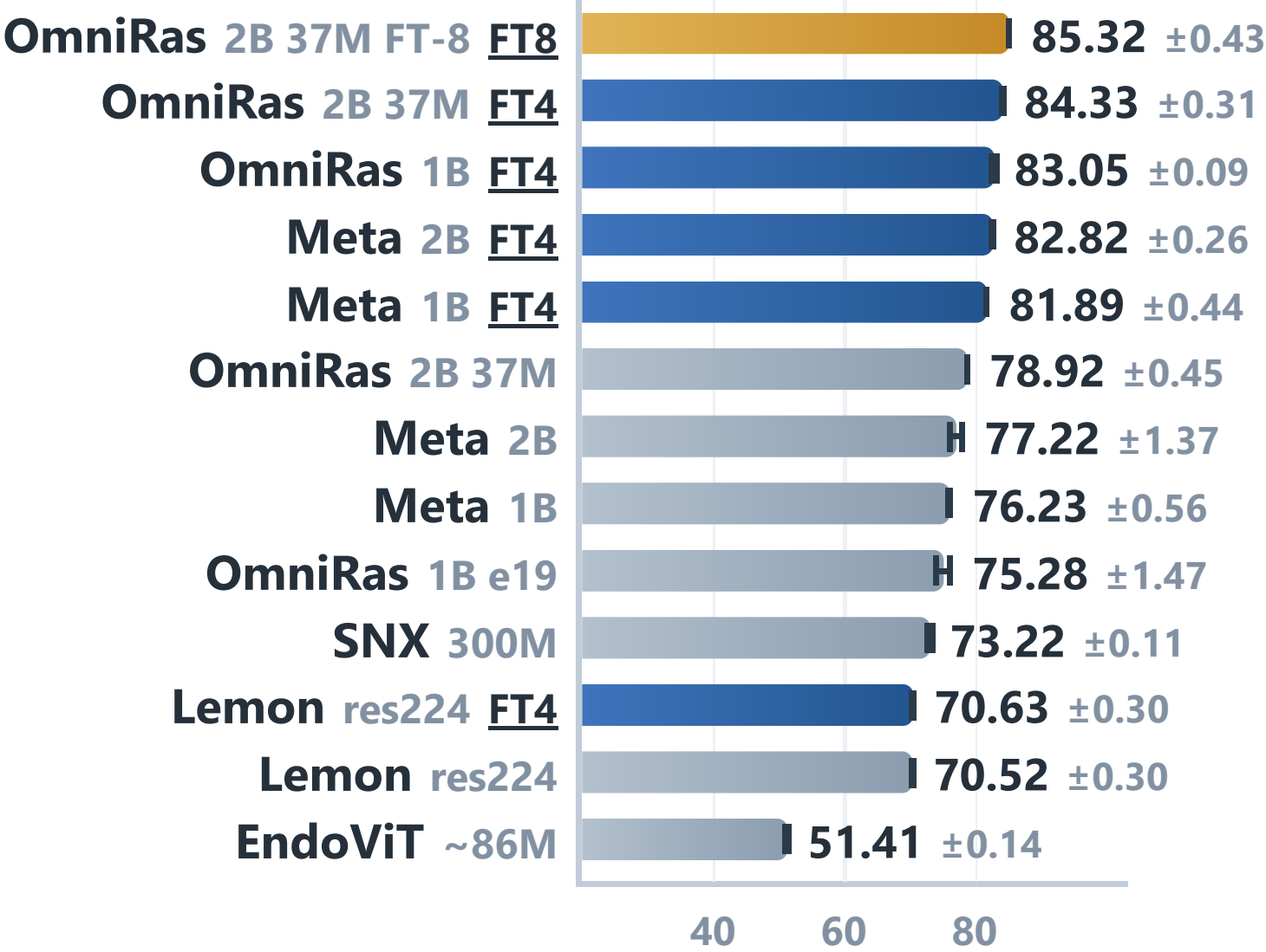
Verb mAP
